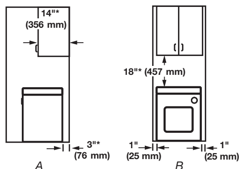
A. Side view - closet or confined area
